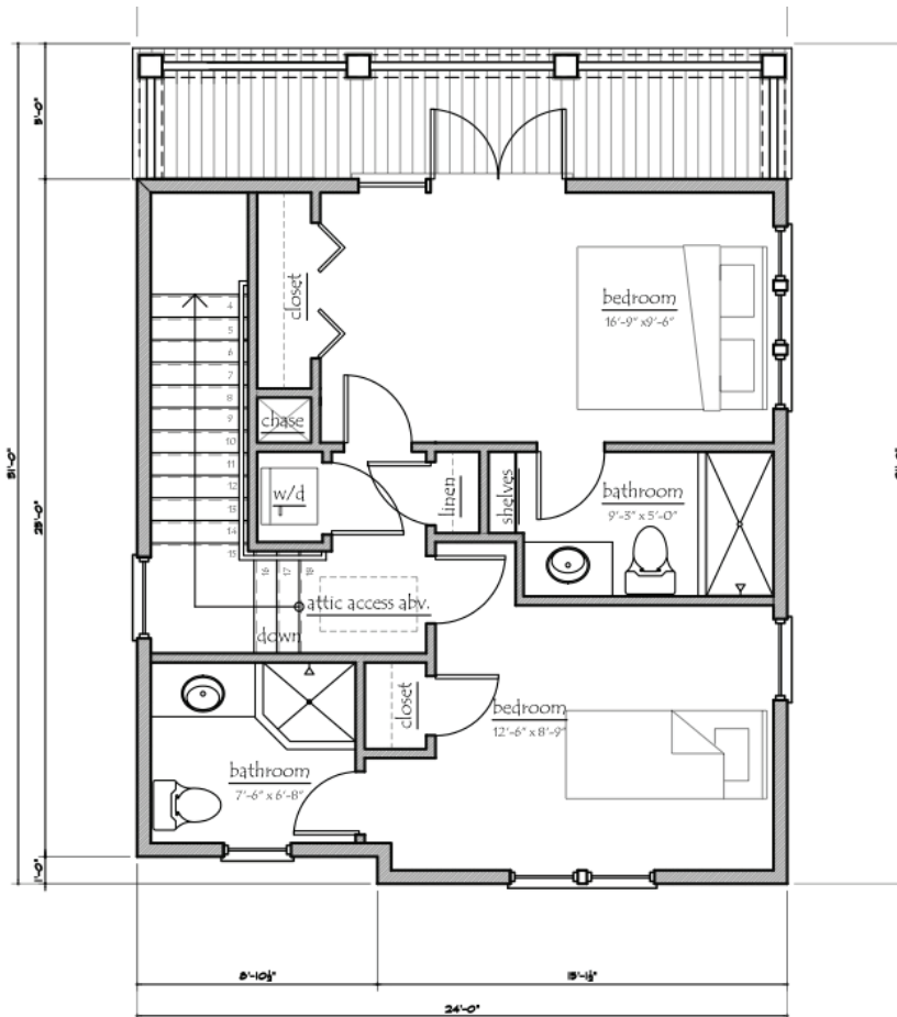
2st floor (614 sq. ft.) balcony (120 sq. ft.)
