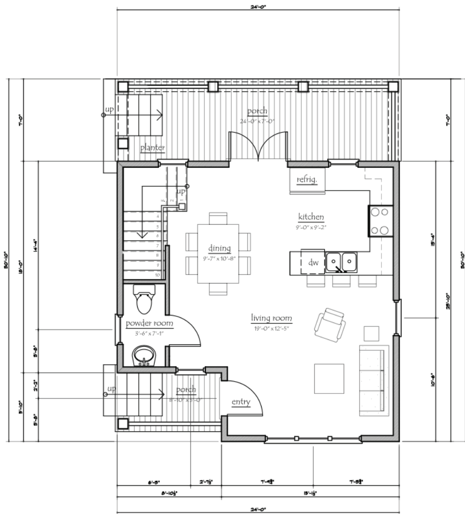
1st floor (520 sq. ft.) porches (212.37 sq. ft.)
